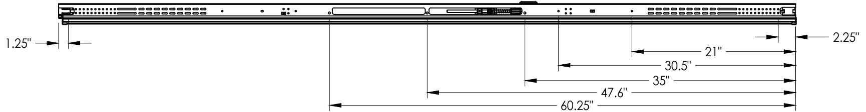
ANCHOR SCREW LOCATIONS
